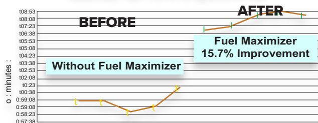
SAE J1321 Fuel Consumption Test Results Engine Tested Cummins N14 with #2 Sinclair Diesel Stationary Test 1 oz to 23 gallons of fuel
